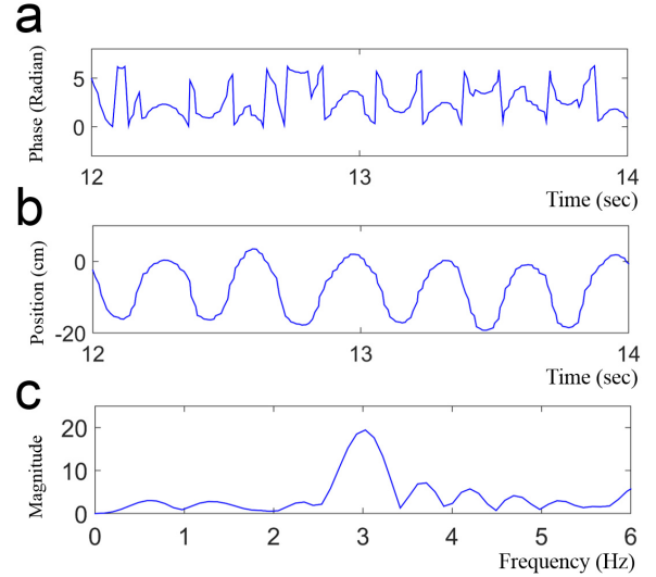
Figure 5. (a) Two segments of raw phase data; (b) application of the trace recovering technique to reveal the moving trace relative to the RFID reader; (c) applying a Fast Fourier transform to reveal the frequency of the movement.
